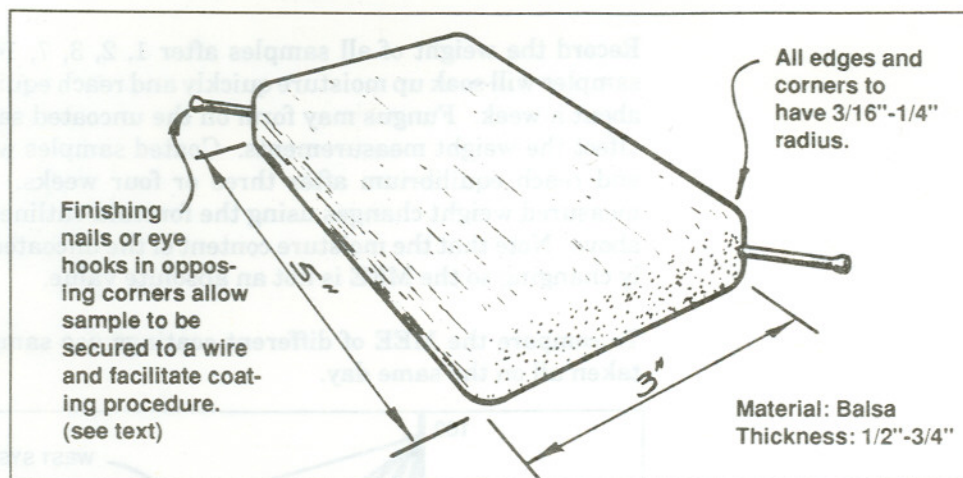
Figure 1 Moisture Exclusion Effectiveness Test Sample
