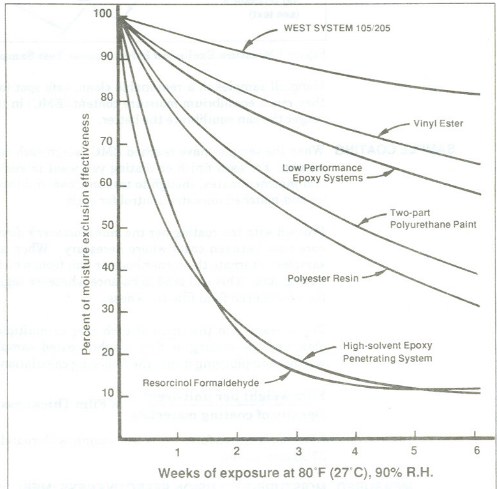
Figure 1 Moisture Exclusion Effectiveness of Various Marine Coatings
